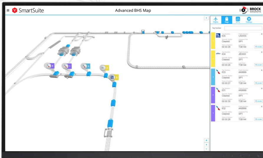
Screenshots of the Advanced BHS Map module on the web client and Mobile HMI on mobile to access the BHS network remotely.
